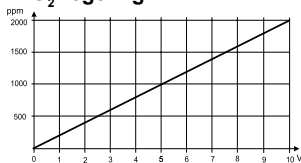
Diagram CO 2 -sensor
